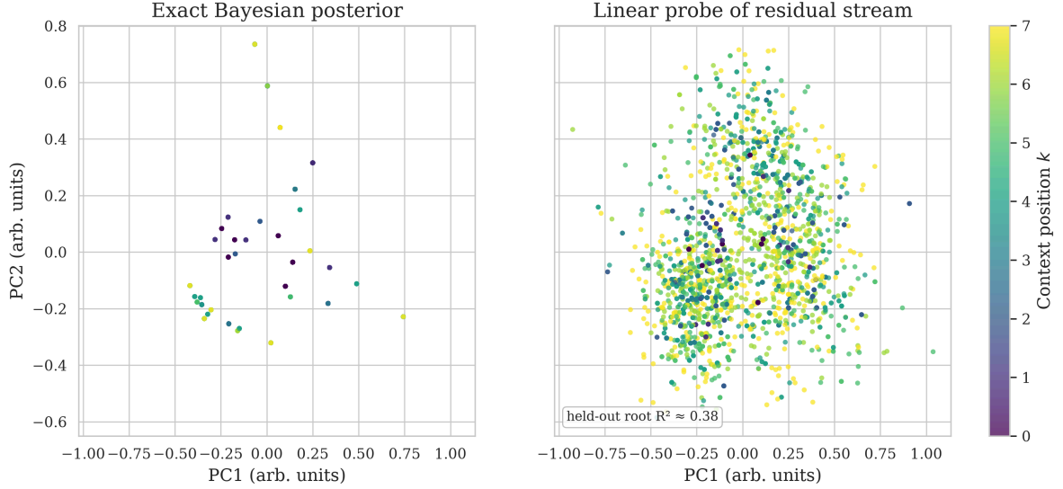
Figure 2: The residual stream is an affine image of the exact belief simplex. Left: PCA(2) of the exact root posteriors; small- k points sit near the prior, large- k points spread toward vertices. Right: the linear probe’s predictions in the same basis, colored by context position — same region, same gradient, recovered at R^2 \approx 0.38 .
