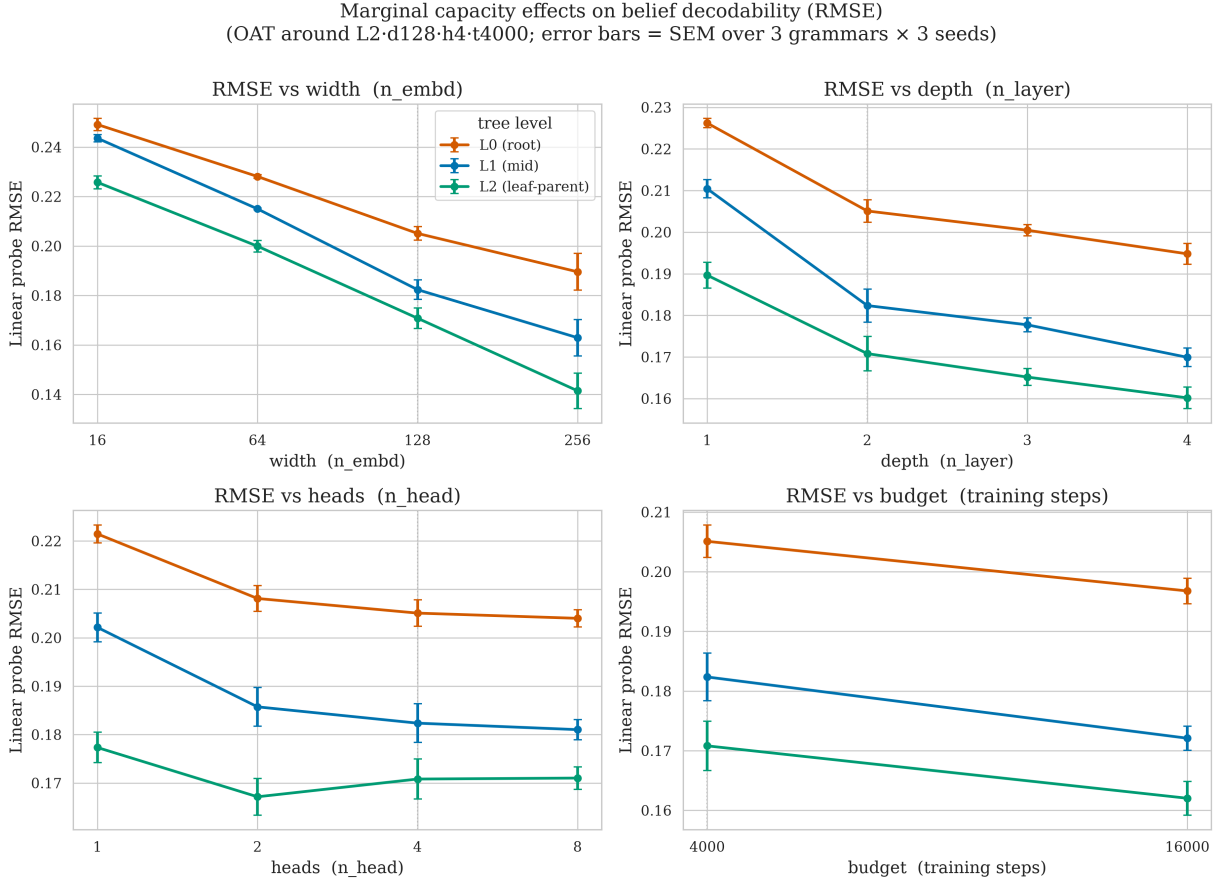
Figure 30: Marginal effects of width, depth, heads, and training budget on probe RMSE — RMSE counterpart of Figure 14.
