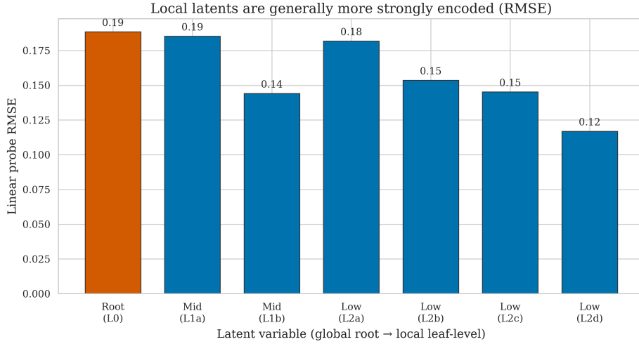
Figure 25: Per-latent probe RMSE on the canonical run — the RMSE counterpart of Figure 4. RMSE is generally lower (better) for the deeper latents, mirroring the R^2 gradient, but is not its exact reflection because each latent’s posterior has a different scale.
