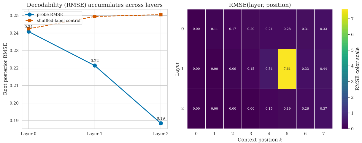
Figure 26: Root-probe RMSE across residual depth and context — the RMSE counterpart of Figure 3. Left: RMSE falls across the three readout points while the shuffled control stays high. Right: the (readout point, position) RMSE heatmap (autoscaled).
