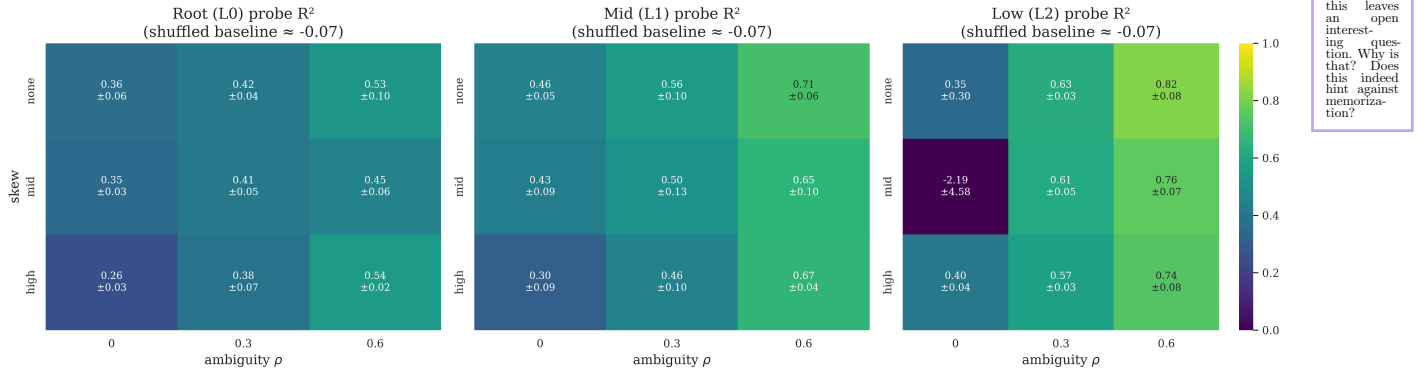
Figure 9: The linear probe survives ambiguity and skew, and sharpens with ambiguity. Per-level probe R^2 (root L_0 , mid L_1 , low L_2 ) over the 3 \times 3 skew \times ambiguity grid; each cell is mean \pm SD over 3 rule-table draws, against a shuffled baseline of \approx -0.07 . R^2 rises left-to-right (with \rho ) at every level. The single dark L_2 cell at (mid, \rho=0 ) is a near-deterministic-target instability, not a decodability failure.
