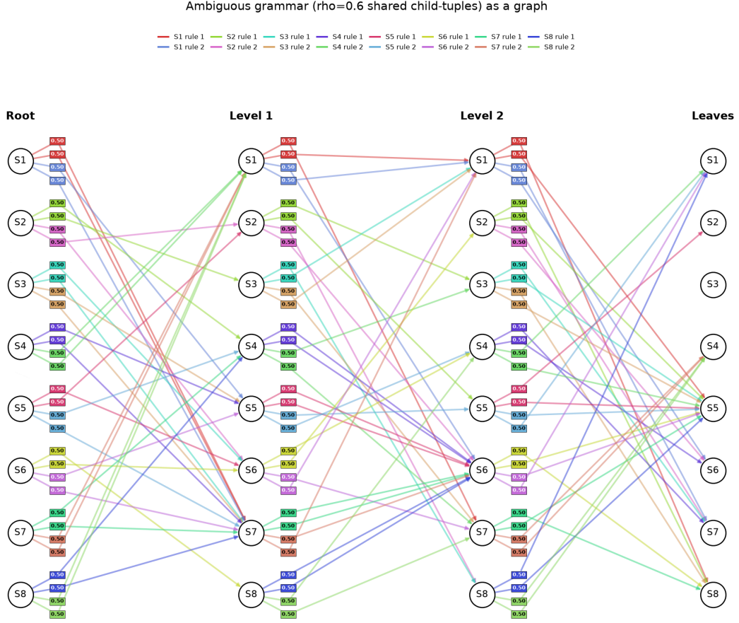
Figure 24: The ambiguous grammar as a DAG. Rule-choice probabilities are uniform, but child-tuples are shared across parents’ rules’ parents’ rules (bold cells in the table; edges converging on the same node in the graph) – the many-to-one structure that makes the belief non-collapsing.
