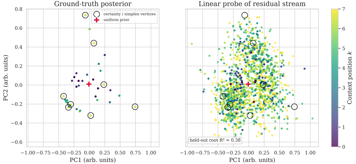
Figure 2: The residual stream is a partial affine image of the exact belief simplex. Left: PCA(2) of the ground truth root posteriors (few distinct values, hence sharp overplotted dots); small- k points sit near the prior, large- k points spread toward vertices. Right: the linear probe’s predictions in the same basis, colored by context position — the same region and position gradient, but a diffuse cloud: held-out root R^2 \approx 0.38 , an imperfect recovery, not an exact one.
