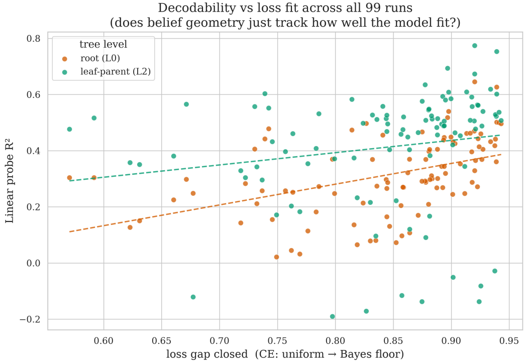
Figure 16: Decodability vs loss fit, all 99 runs. Root ( L_0 ) and leaf-parent ( L_2 ) probe R^2 against loss_gap_closed (fraction of the uniform \rightarrow Bayes CE gap closed). Dashed lines are least-squares fits; the wide vertical spread at fixed loss fit shows decodability is not determined by how well the model fit the loss.
