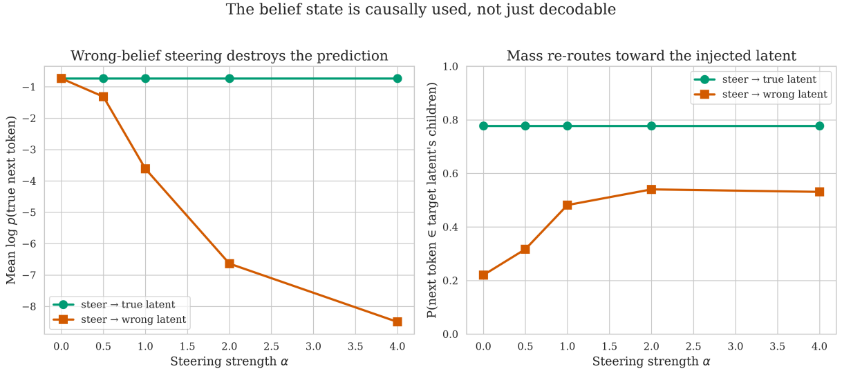
Figure 6: The belief state is causally used. Steering the layer-1 residual toward the true latent leaves predictions intact (green); steering toward a wrong latent collapses the true next token’s log-probability (left, orange: -0.73 \rightarrow -8.5 ) and re-routes mass onto the wrong latent’s children (right, orange: 0.22 \rightarrow 0.53 ).
