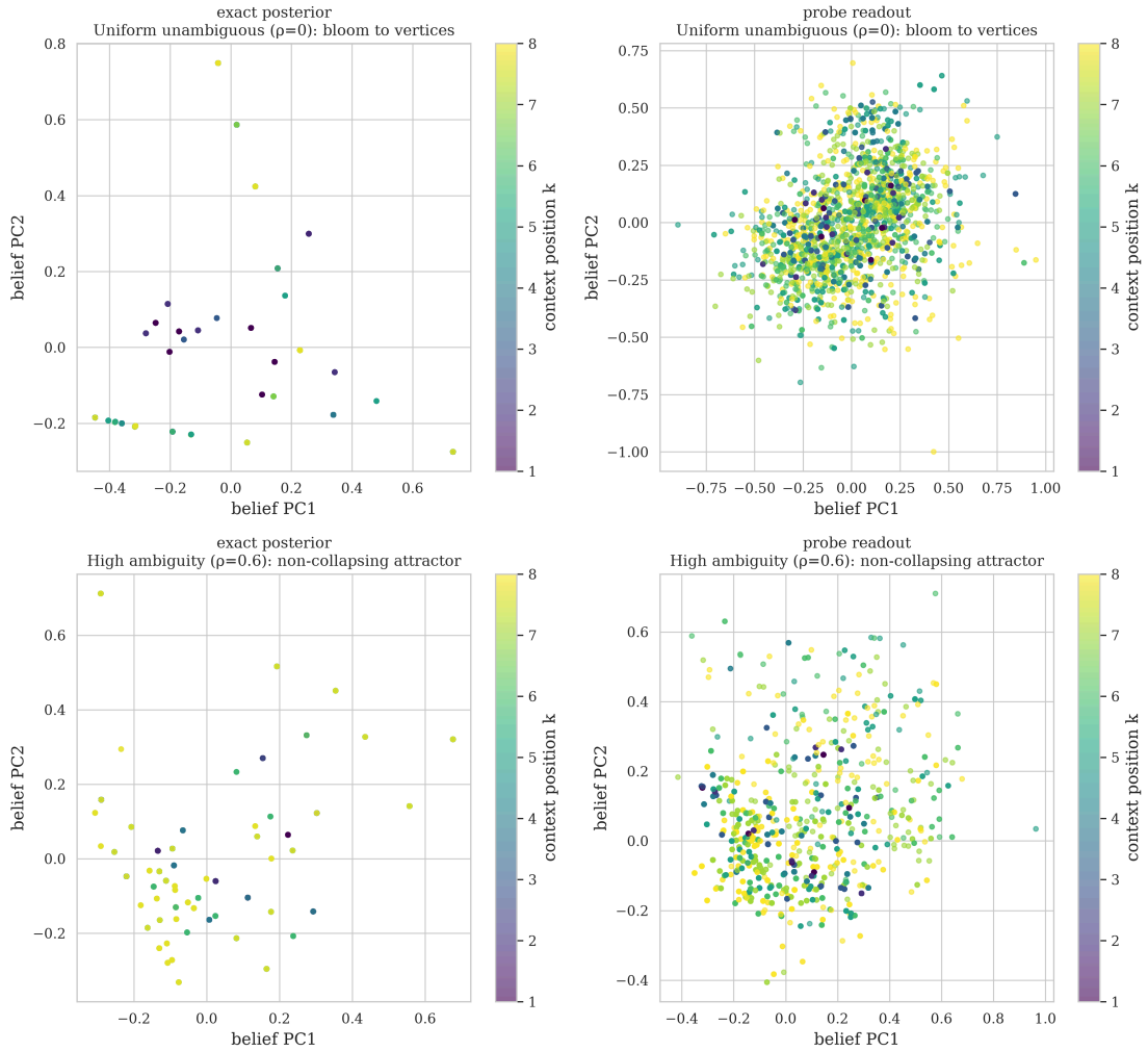
Figure 10: Exact posterior (left column) and linear-probe readout (right column) in belief-PCA, colored by context position, for the uniform corner \rho = 0 (top) and the high-ambiguity corner \rho = 0.6 (bottom). At \rho = 0 the late-context beliefs reach the simplex vertices (bloom-to-certainty); at \rho = 0.6 they form a structured interior cloud — the non-collapsing attractor — which the probe readout traces.
