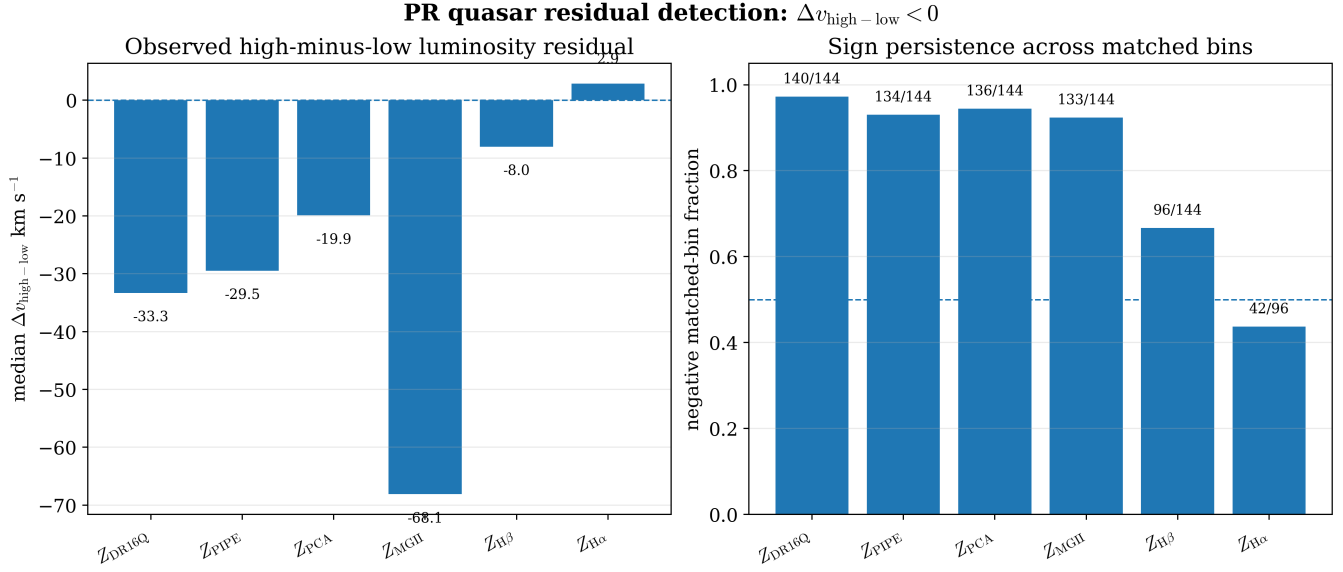
Figure 4: PR-native quasar residual detection: \Delta v_{\text{high} - \text{low}} < 0 . Observed velocity residuals between high- and low-luminosity subsamples across matched-redshift bins. The predicted negative contrast is statistically robust across independent estimators ( Z_{\text{DR16Q}} , Z_{\text{PIPE}} , Z_{\text{PCA}} , Z_{\text{MGII}} ) and survives strict low-ionization anchoring, warning-clean cuts, random-label permutations, and bootstrap resampling.
