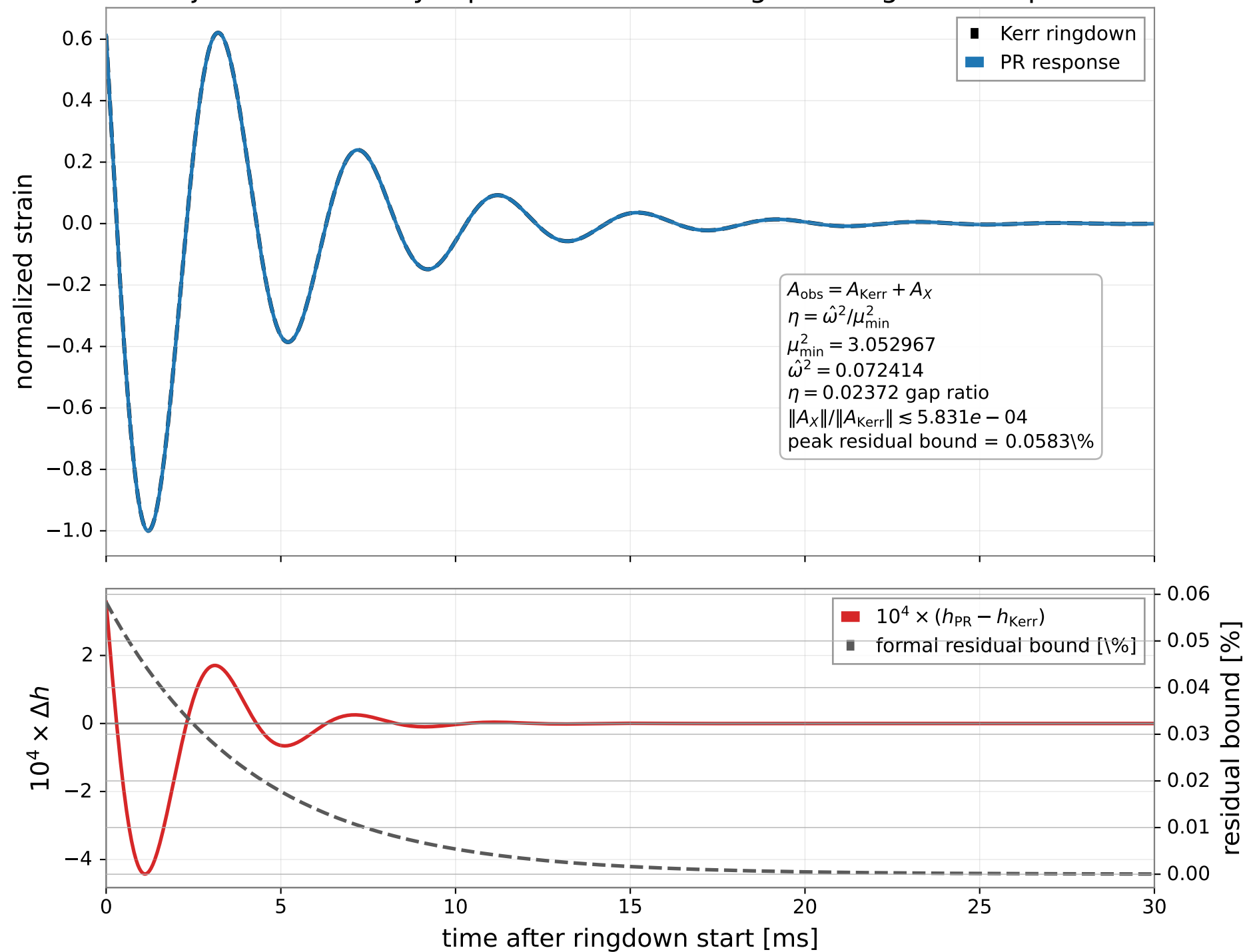
Projection Relativity reproduces the leading Kerr ringdown response
