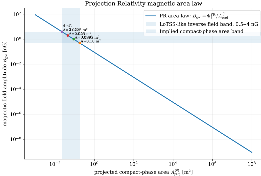
Figure 5: Projection Relativity magnetic area law. The compact phase sector fixes the flux normalization \Phi_\theta^{\text{PR}} = (\hbar/e)(Z_A/c_{bc}) , while the realized magnetic domain supplies the projected compact-phase area A_{\text{proj}}^{(\theta)} . The resulting field is B_{\text{geo}}^{\text{PR}}[\text{nG}] = 0.09009597185/A_{\text{proj}}^{(\theta)}[\text{m}^2] . The shaded band shows the compact-phase areas corresponding to the foreground-cleaned LoTSS-scale residual field range.
