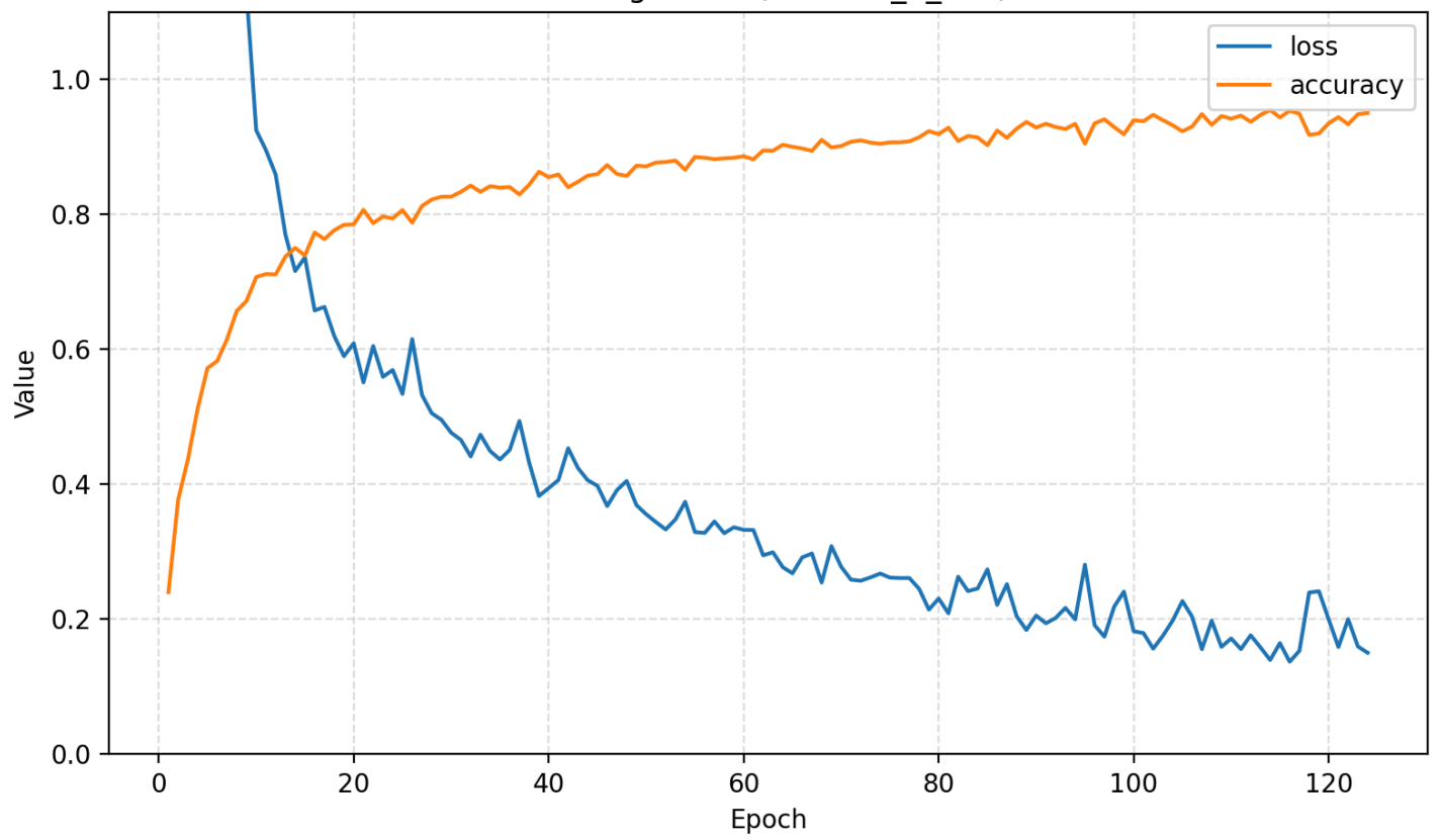
Training Curve (Baltrum_S_FP1)
