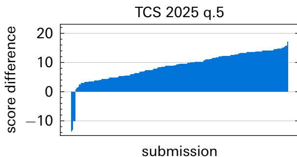
Figure 10: Difference in human and automatic grading for the TCS 2025 dataset, question 5. Sorted by increasing difference.
