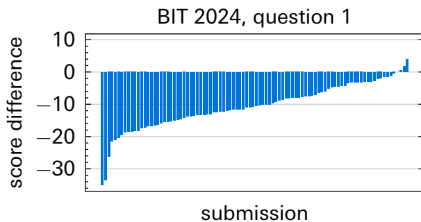
Figure 9: Difference in grades in the BIT 2024 dataset. Sorted by increasing difference.
