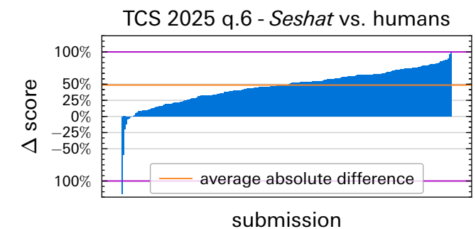
Figure 23: Difference in human and Seshat grading for the TCS 2025 dataset, question 6. Normalised to the maximum points in the rubric and sorted by increasing difference. Positive scores mean that Seshat awarded more points.
