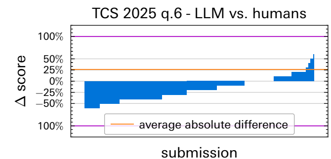
Figure 24: Difference in human and LLM grading for the TCS 2025 dataset, question 6. Normalised to the maximum points in the rubric and sorted by increasing difference. Positive scores mean that Seshat awarded more points.
