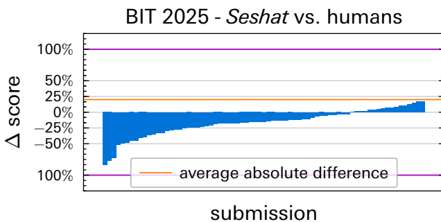
Figure 28: Difference in human and Seshat grading for the BIT 2025 dataset, question 6. Normalised to the maximum points in the rubric and sorted by increasing difference. Positive scores mean that Seshat awarded more points.
