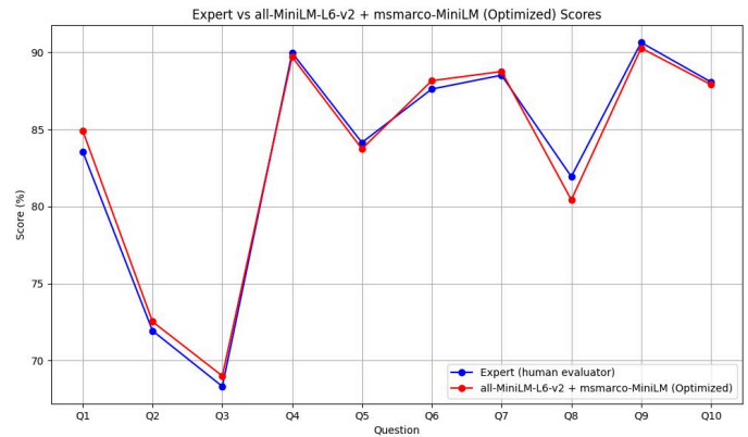
Figure 5: R. Ramachandran et al. [38, p.13] : Comparison of expert scores and CodeLLama scores using a combination of all-MiniLM-L6-v2 and msmarco-MiniLM as word similarity models.
