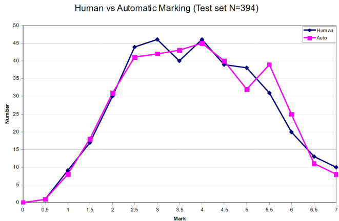
Figure 4: P. Thomas et al. [27, Fig. 3]: Human vs. automatic grading in database ER diagrams.
