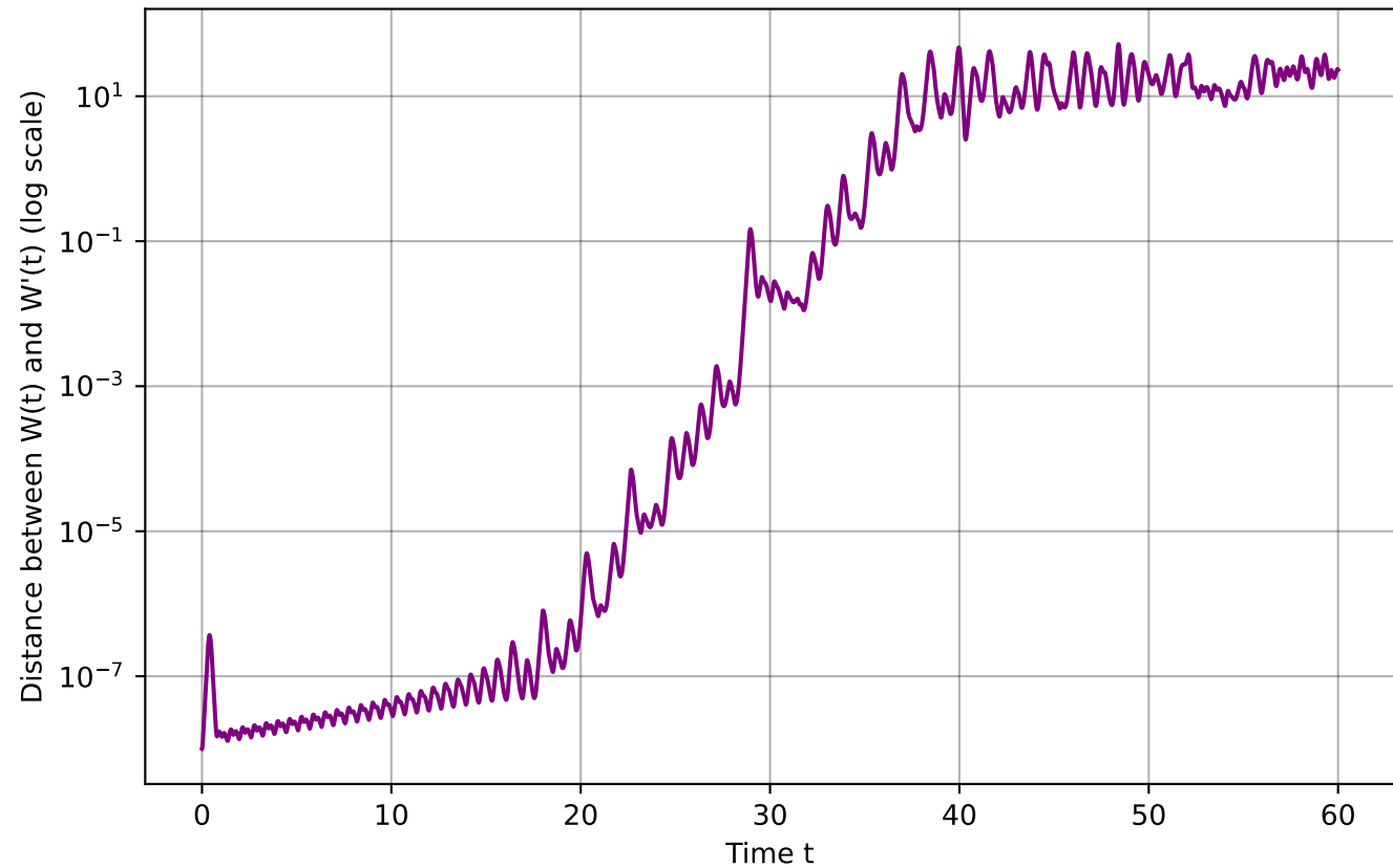
Difference between Solutions to Lorenz Equations vs. Time
