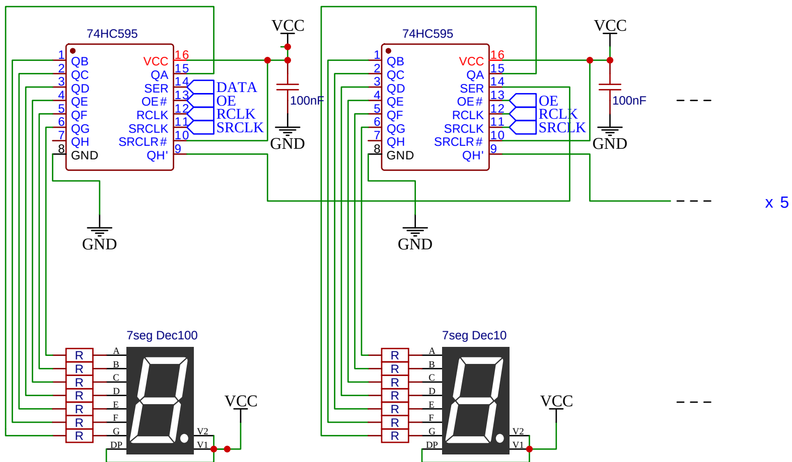
5 Seven segment displays with common anode
