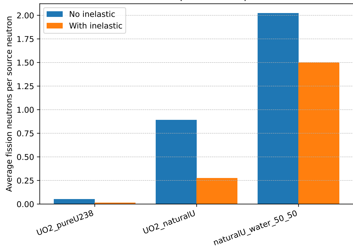
Neutron multiplication comparison
