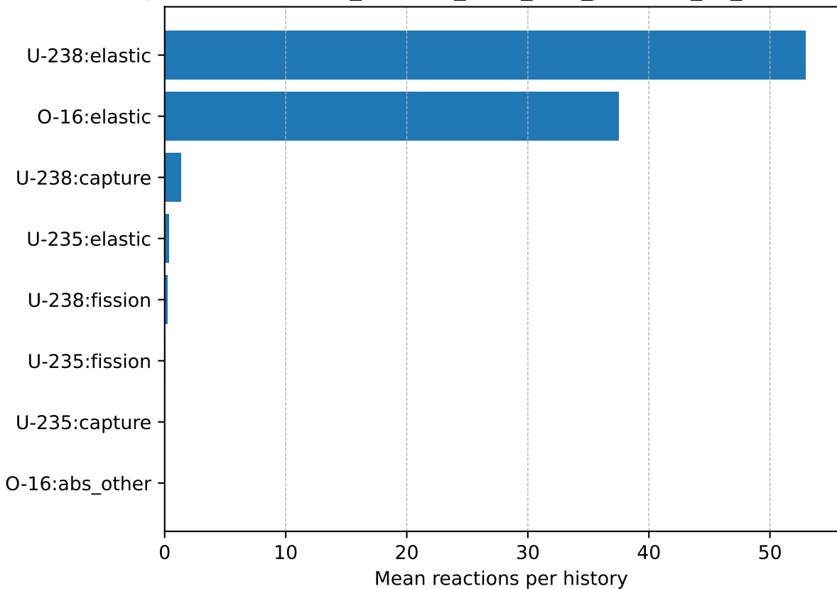
Top reactions — ex2_reaction_stats_UO2_naturalU_no_inelastic.csv
