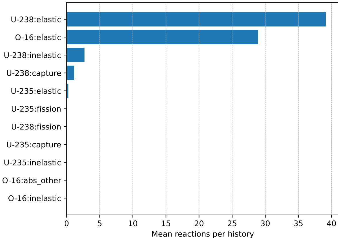
Top reactions — ex2_reaction_stats_UO2_naturalU_with_inelastic.csv
