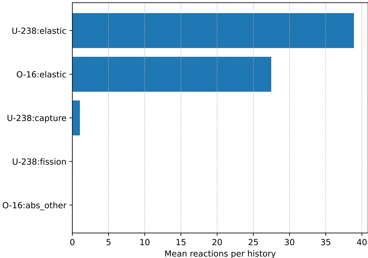
Top reactions — ex2_reaction_stats_UO2_pureU238_no_inelastic.csv
