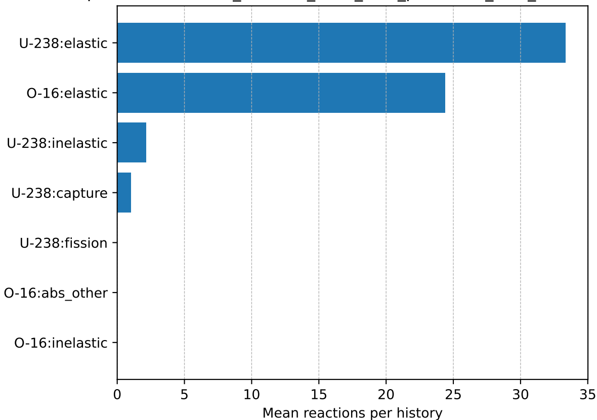
Top reactions — ex2_reaction_stats_UO2_pureU238_with_inelastic.csv
