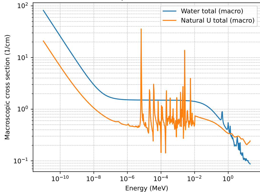
Macroscopic total cross sections
