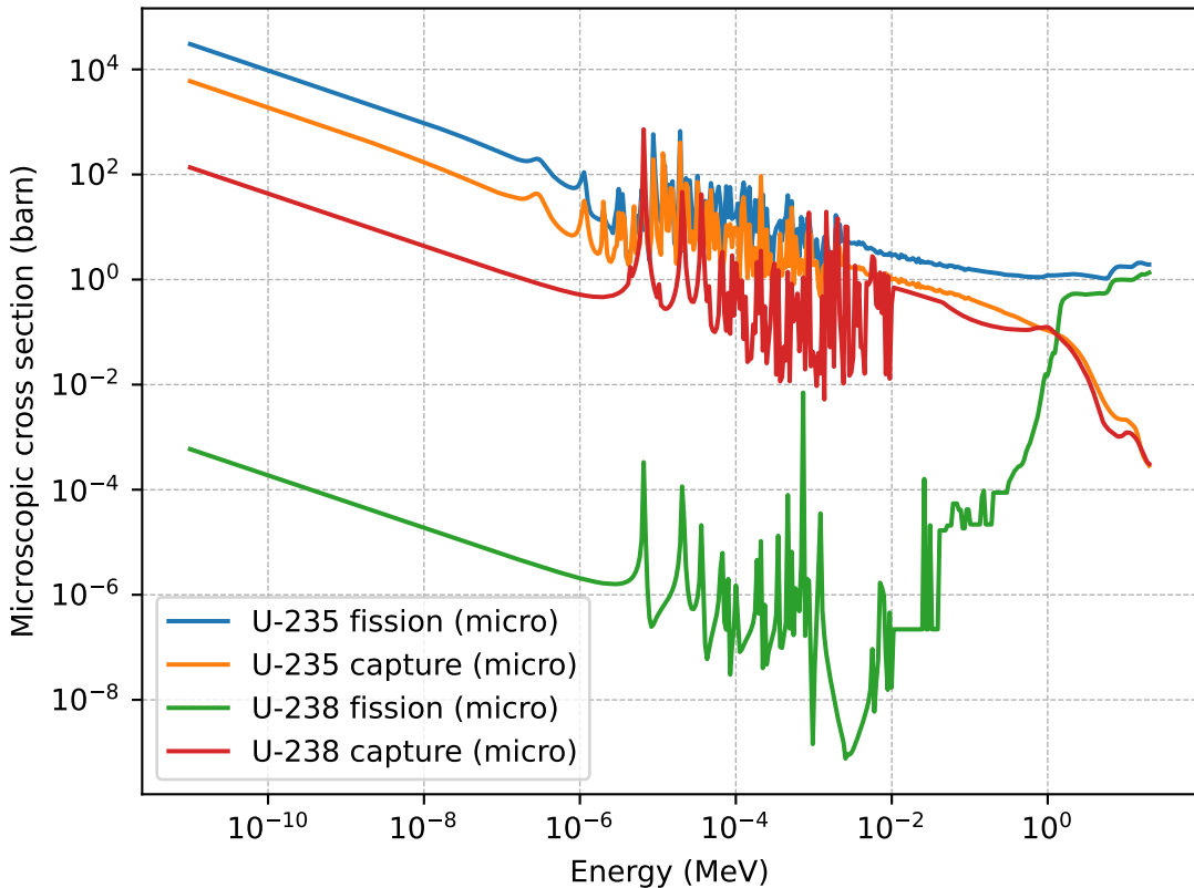
Microscopic fission and capture cross sections
