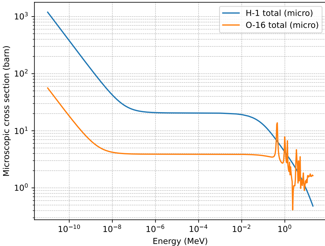
Microscopic total cross sections
