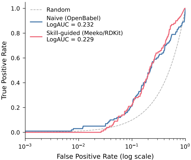
Semi-log ROC Curve
