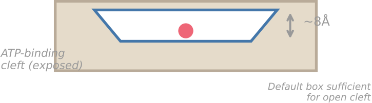
CDK2 (PDB 1H1Q)
