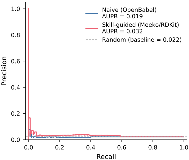
Precision-Recall -- dpp4
