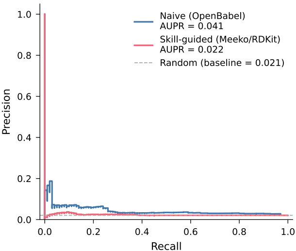
Precision-Recall -- esr1
