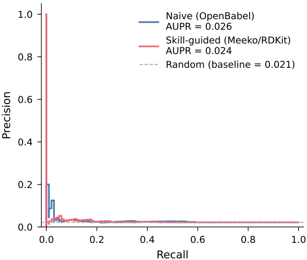
Precision-Recall -- hsp90
