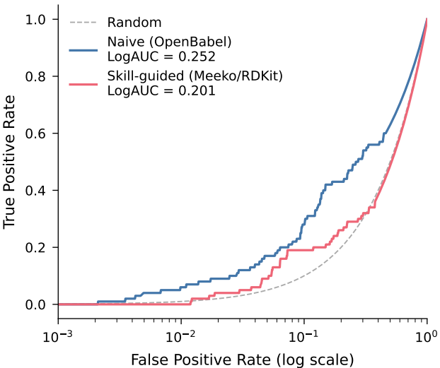
Semi-log ROC -- thrombin
