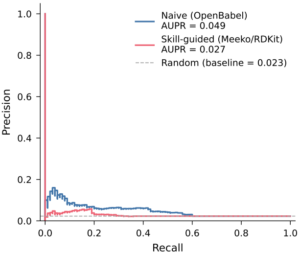
Precision-Recall -- thrombin
