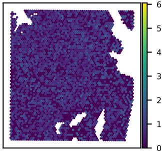
SNU51A SACM1L expression Moran's I = 0.01
