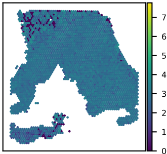
SNU18A TMBIM6 expression Moran's I = 0.17
