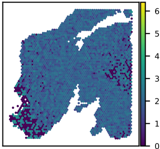
SNU24A COPE expression Moran's I = 0.14
