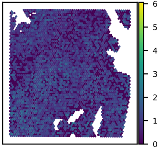
SNU51A SLC35F1 expression Moran's I = 0.10
