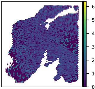
SNU24A HNRNPLL expression Moran's I = 0.07
