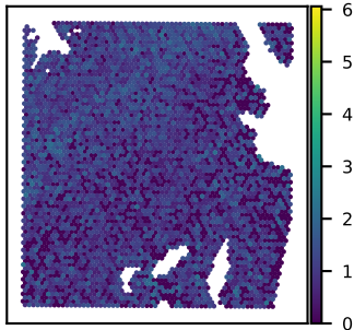
SNU51A SERPINB6 expression Moran's I = 0.08
