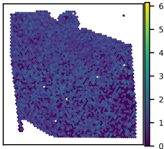
SNU27A SH3GLB1 expression Moran's I = 0.06
