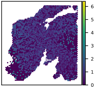
SNU24A CDH20 expression Moran's I = 0.05
