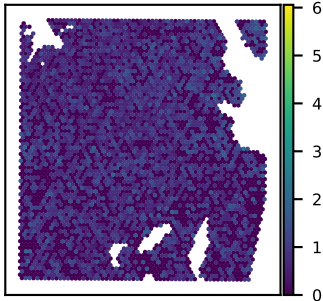
SNU51A UBE2K expression Moran's I = 0.04
