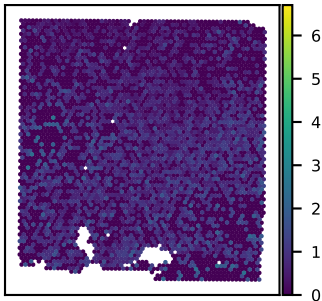
SNU43A HIST1H3A expression Moran's I = 0.07
