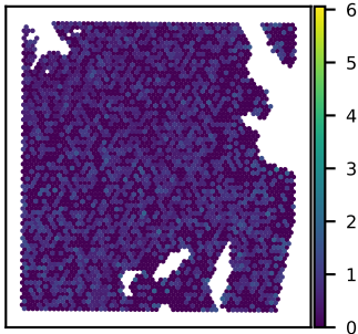
SNU51A PANK4 expression Moran's I = 0.01
