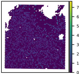
SNU21B SMYD3 expression Moran's I = 0.02
