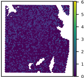
SNU51A OSTF1 expression Moran's I = 0.05
