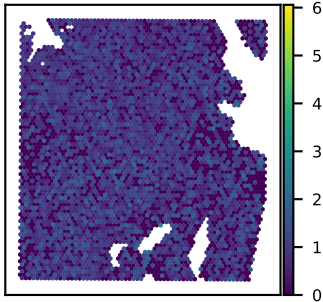
SNU51A PSMD14 expression Moran's I = 0.03
