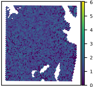
SNU51A RAB11A expression Moran's I = 0.02
