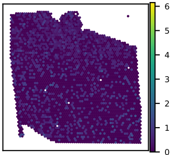
SNU27A TMEM250 expression Moran's I = 0.01
