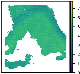
SNU18A TMSB4X expression Moran's I = 0.77
