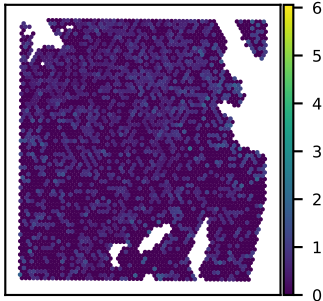
SNU51A FAM13A expression Moran's I = 0.03
