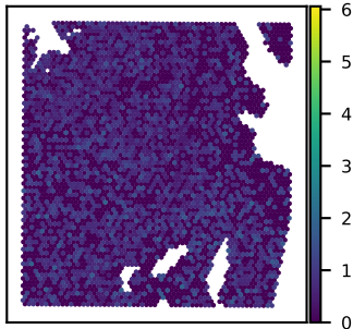
SNU51A TRAFD1 expression Moran's I = 0.03
