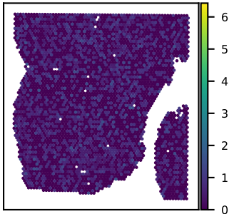
SNU25B KIAA2026 expression Moran's I = 0.01
